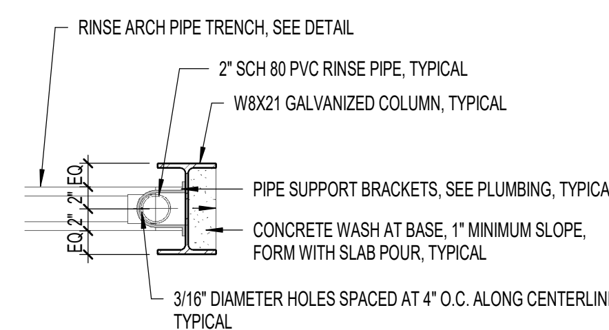
7 DETAIL
