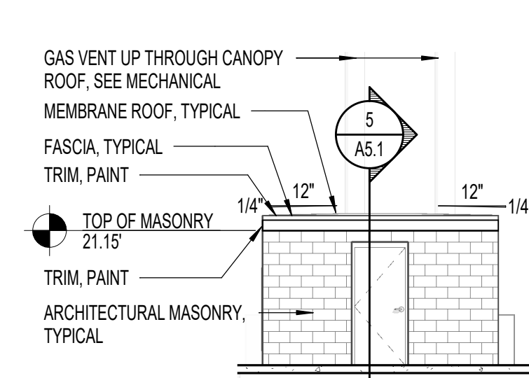
8 WASH - FRONT ELEV
