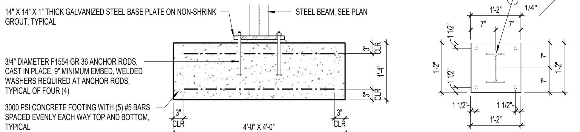
2 RINSE ARCH COLUMN FOOTING
