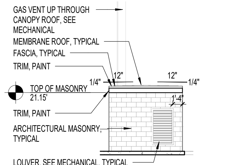
11 WASH - LEFT ELEV
