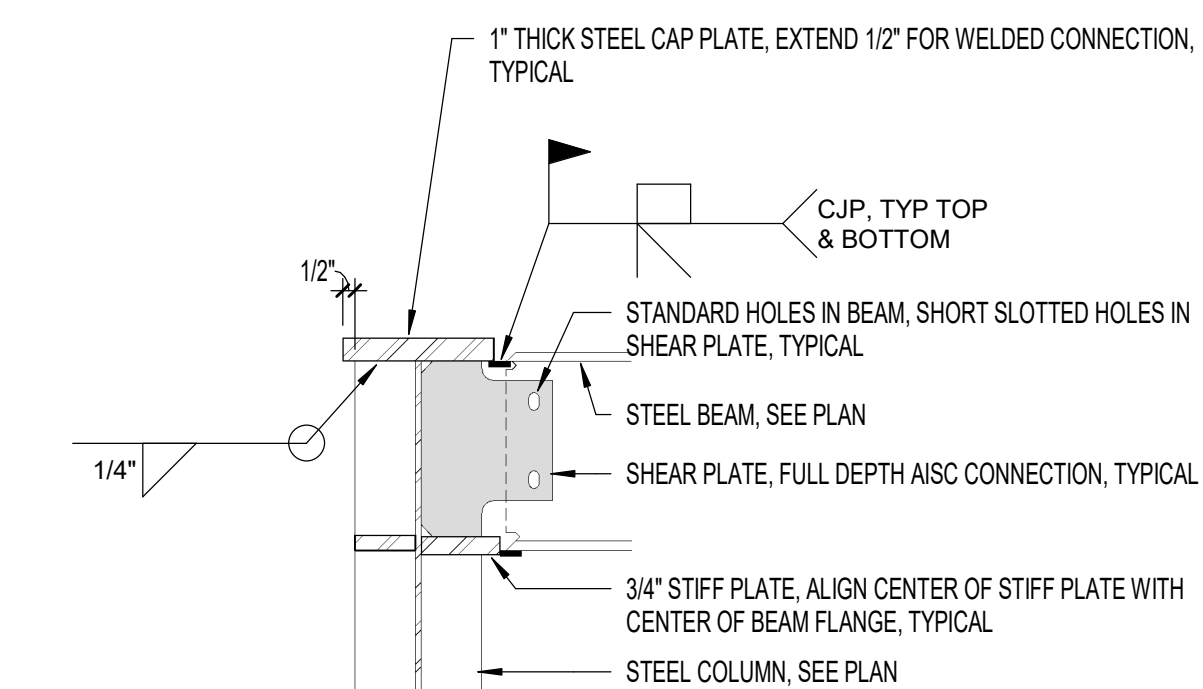
BEAM CONNECTION - SECTION VIEW
