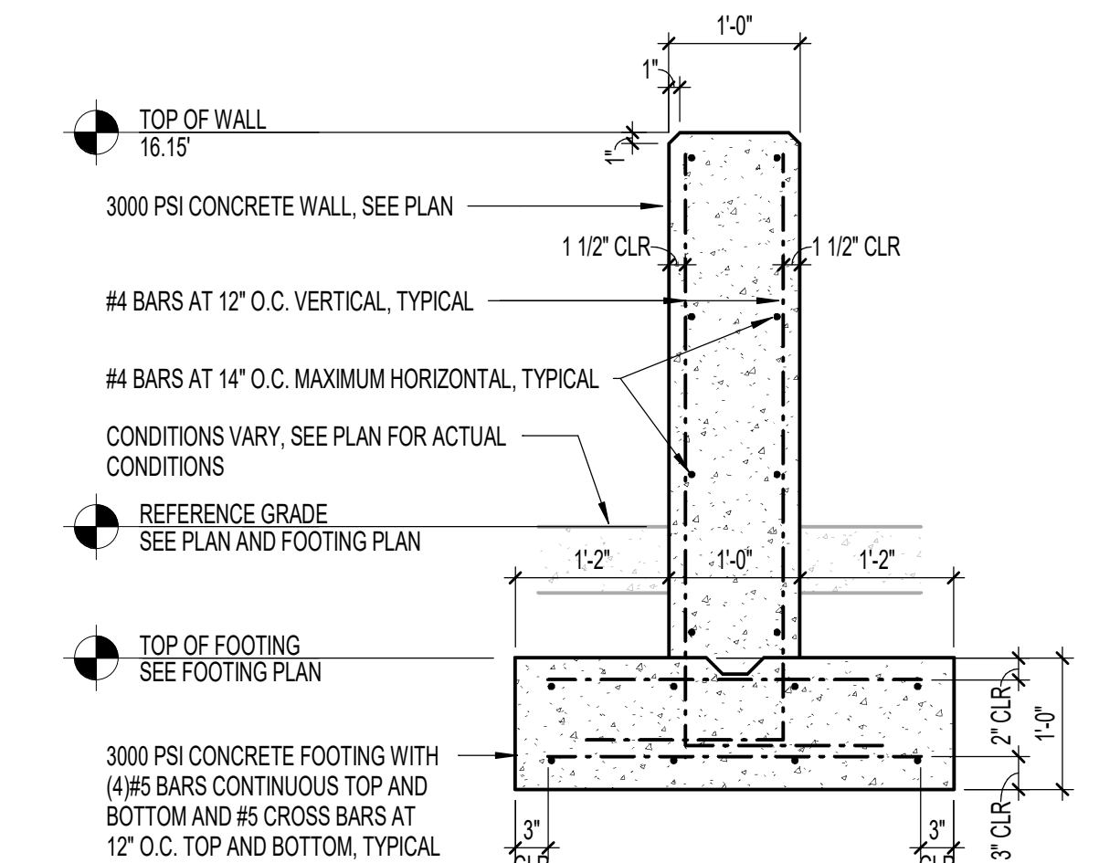
3 CONCRETE WALL
