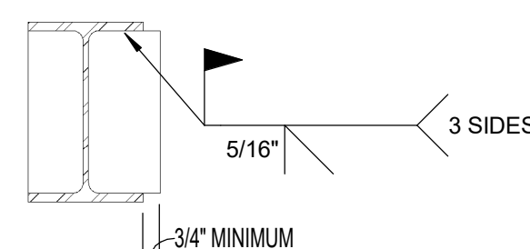
BEAM CONNECTION - SECTION VIEW
