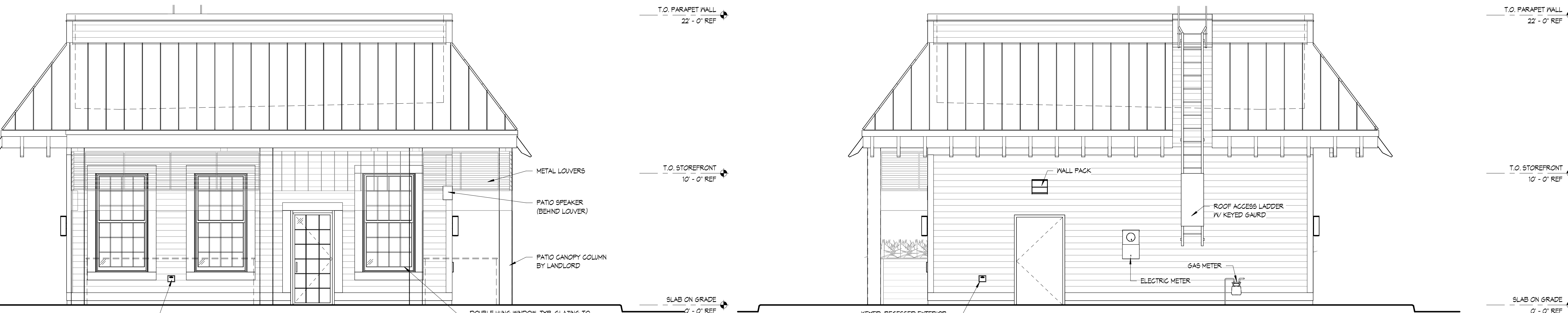
3 PATIO ELEVATION 1/4" = 1'-0"
