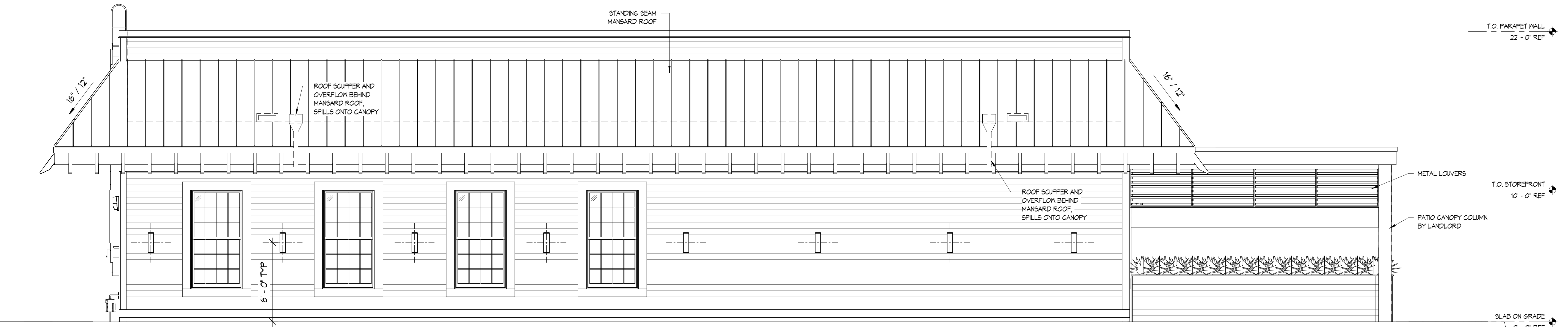
2 STREET ELEVATION 1/4" = 1'-0"
