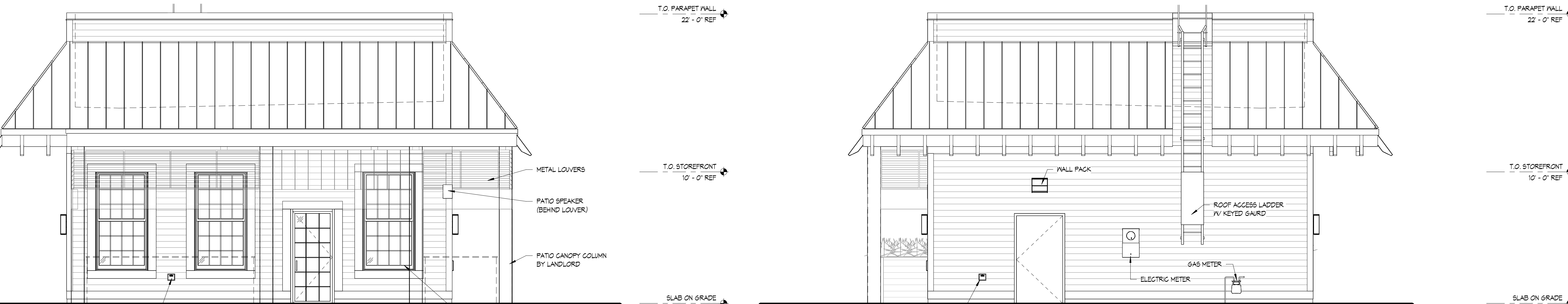
2 STREET ELEVATION 1/4" = 1'-0"
